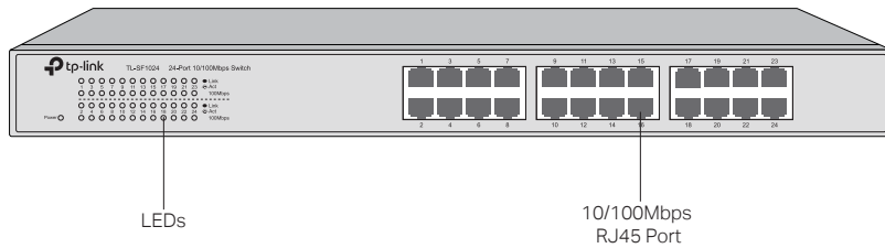
Figure 1-3 Front Panel of TL-SF1024
